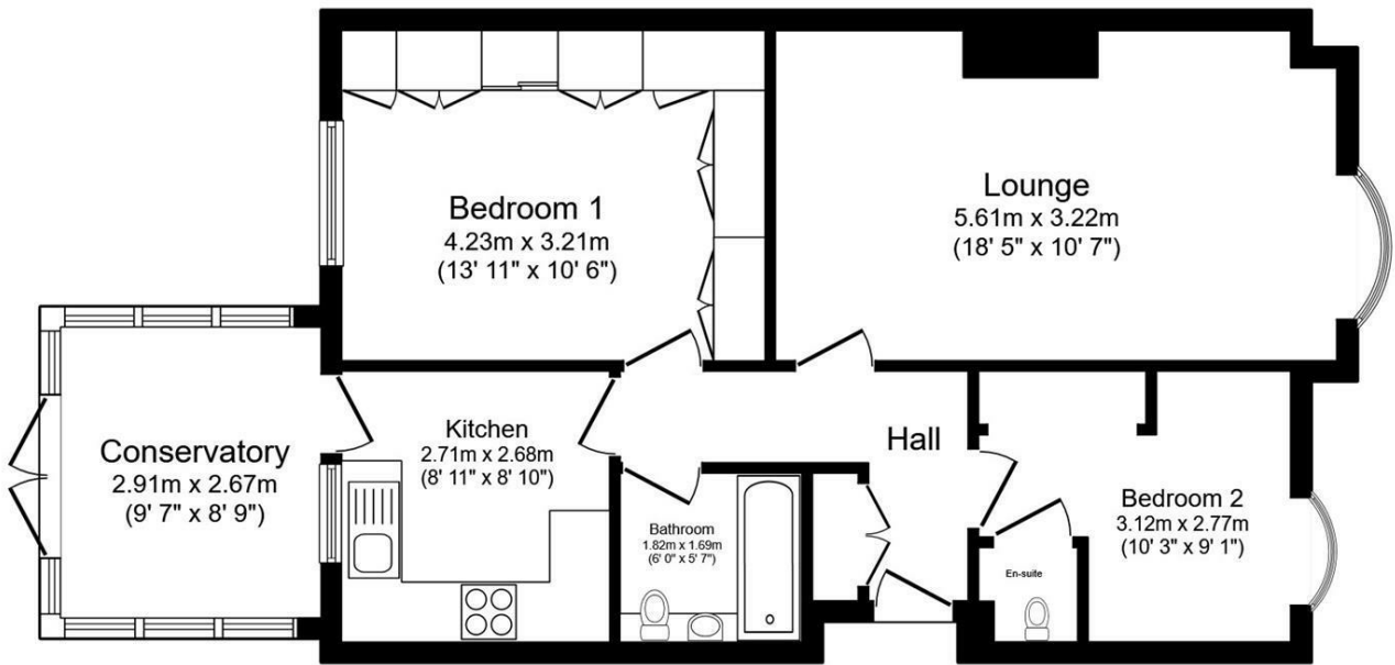
Floor Plan
